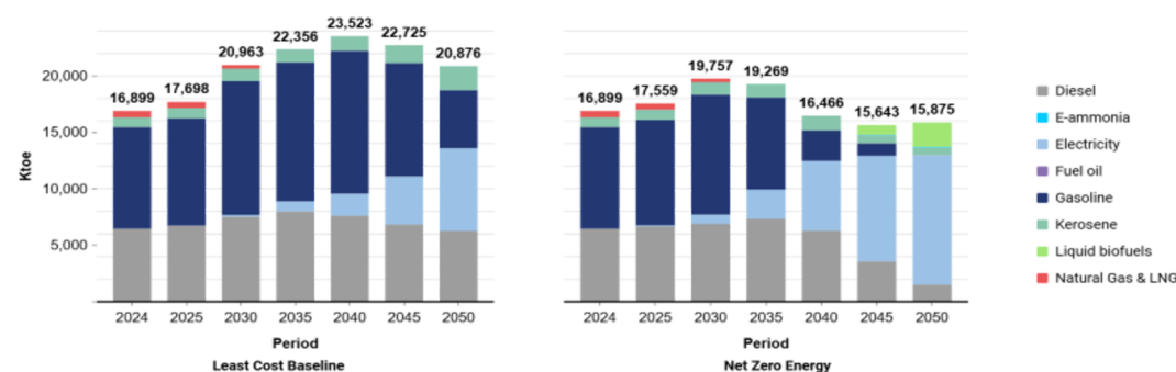
Figure 23: Final Energy Consumption in transport by energy carrier
