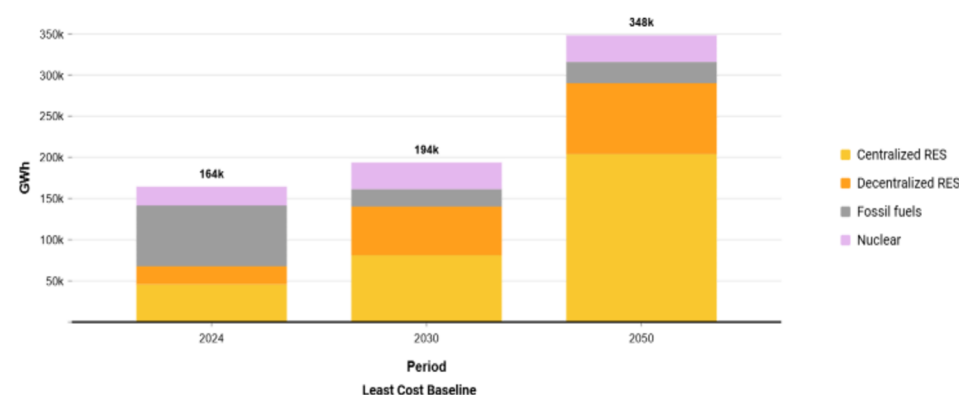
Figure 5: Power generation mix (LCB)
