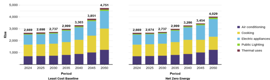
Figure 20: Final Energy Consumption in commercial sector by service
