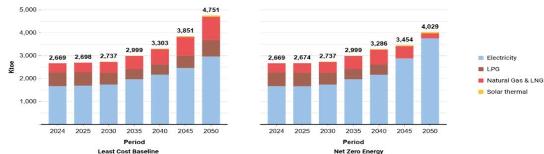
Figure 19: Final Energy Consumption in commercial sector by energy carrier
