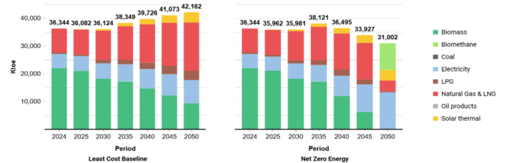
Figure 17: Final Energy Consumption in households by energy carrier
