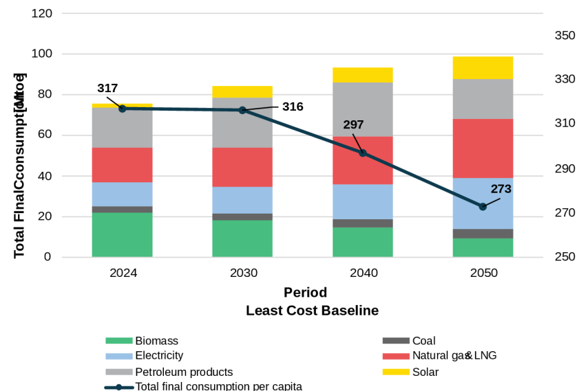
Figure 6: Evolution of Final Energy Consumption by Energy Carrier and per Capita
