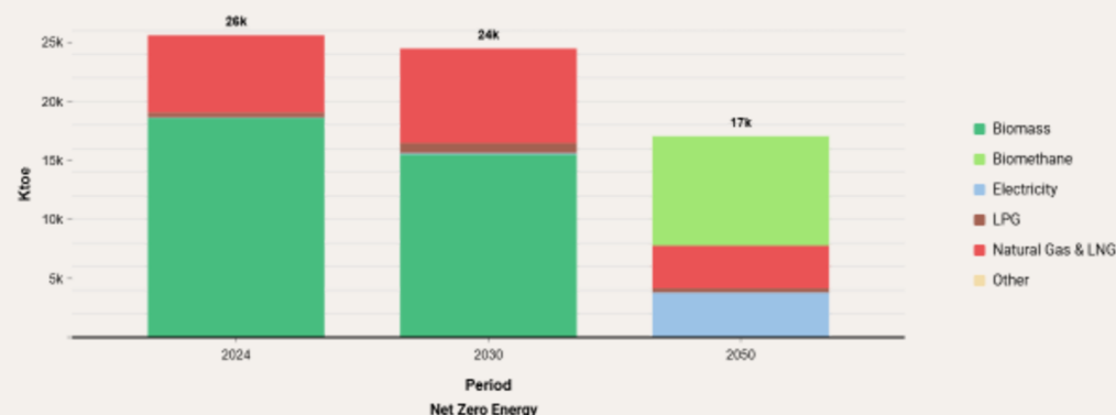
Figure 13: Energy consumption for Residential cooking (NZE)
