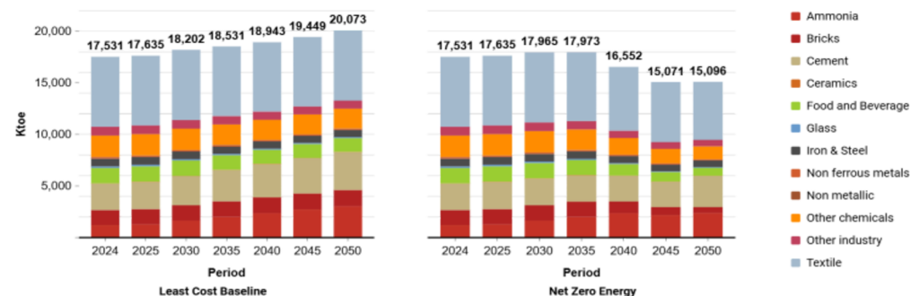
Figure 22: Final Energy Consumption in industry by industrial subsector
